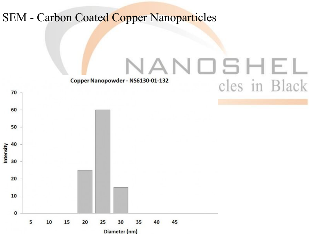
Particles Size Analysis - Copper Nanoparticles
