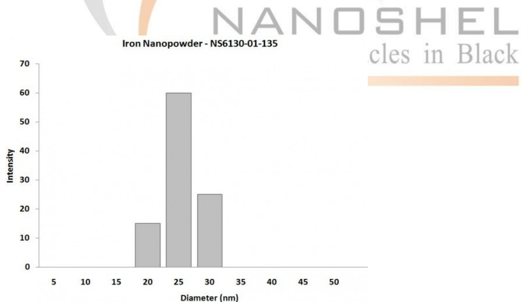
Particles Size Analysis - Fe Nanopowder
