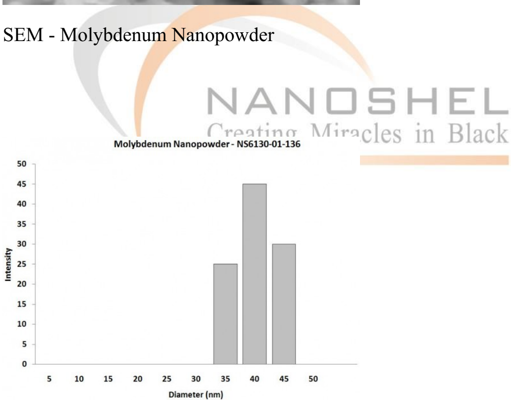
Particles Size Analysis - Mo Nanoparticles
