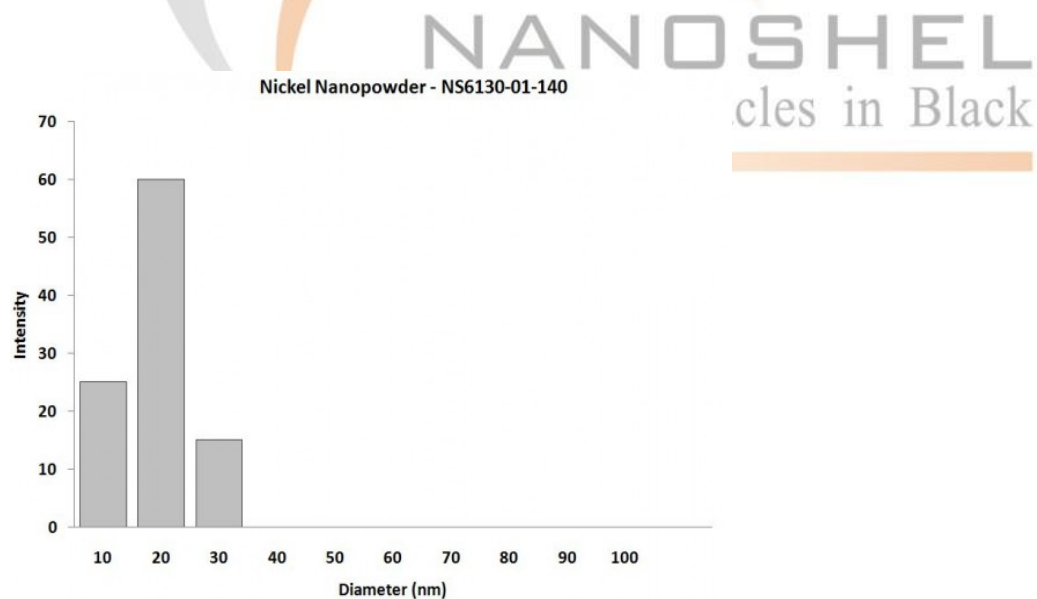
Particles Size Analysis - Ni Nanopowder
