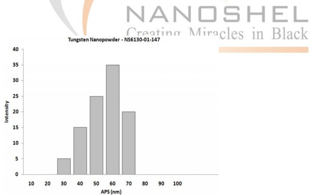
Particles Size Analysis - W Nanopowder
