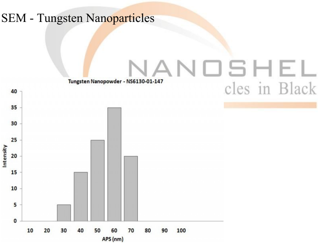
Particles Size Analysis - W Nanopowder
