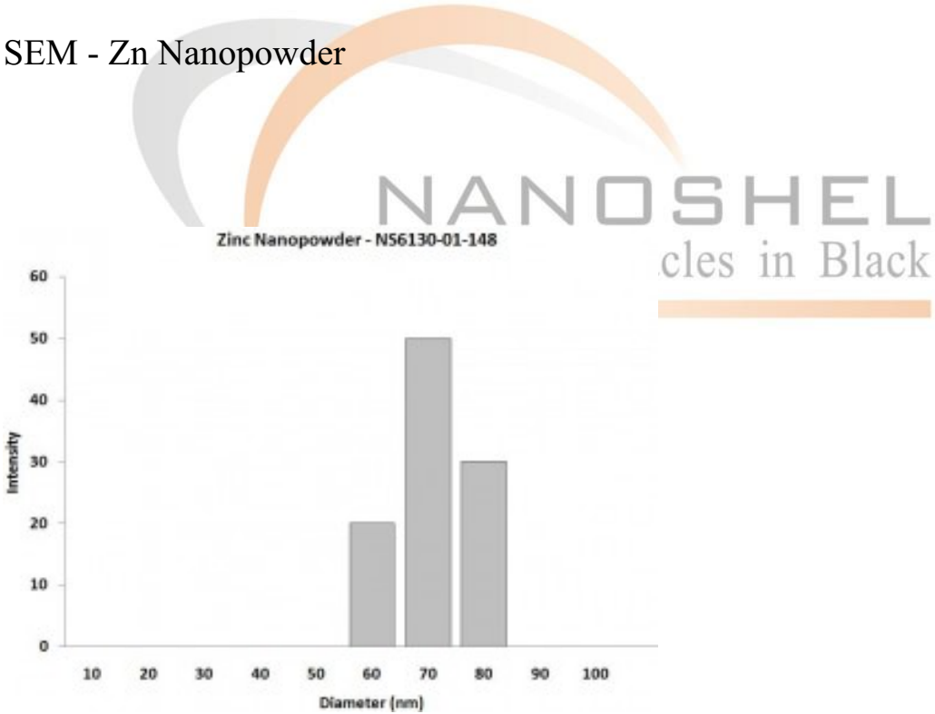
Particles Size Analysis - Zinc Nanopowder
