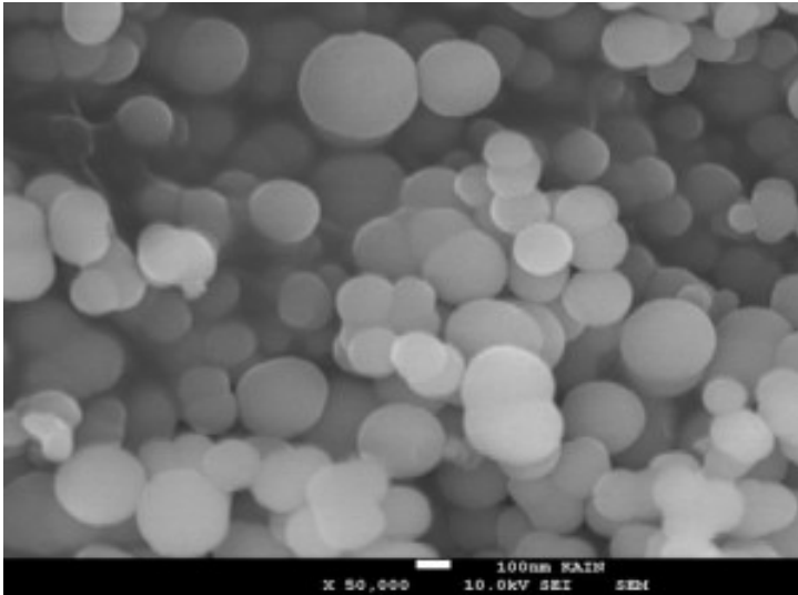
SEM - Cadmium Nanoparticles
