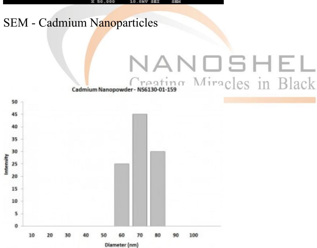
Particles Size Analysis - Cd Nanopowder
