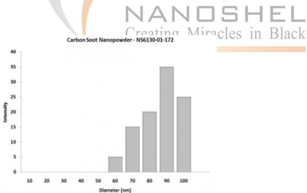
Particles Size Analysis - Carbon Nanoparticles
