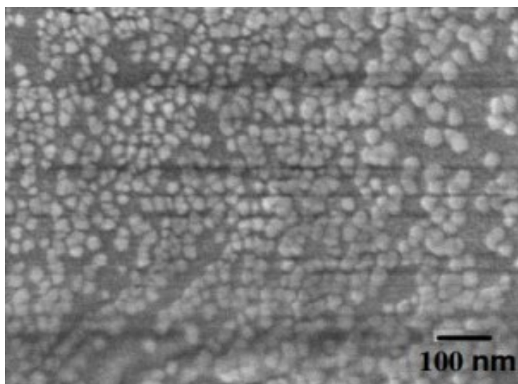
SEM - Soot Carbon Black Nanopowder
