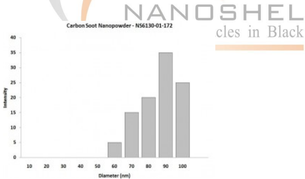
Particles Size Analysis - Carbon Nanoparticles
