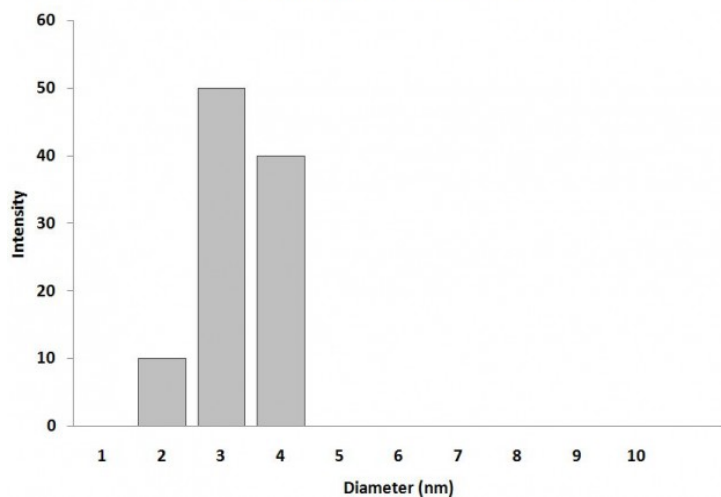
Particles Size Analysis - Graphite Nanoplatelets
