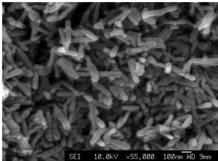
SEM - Hydroxyapatite Nanoparticles
