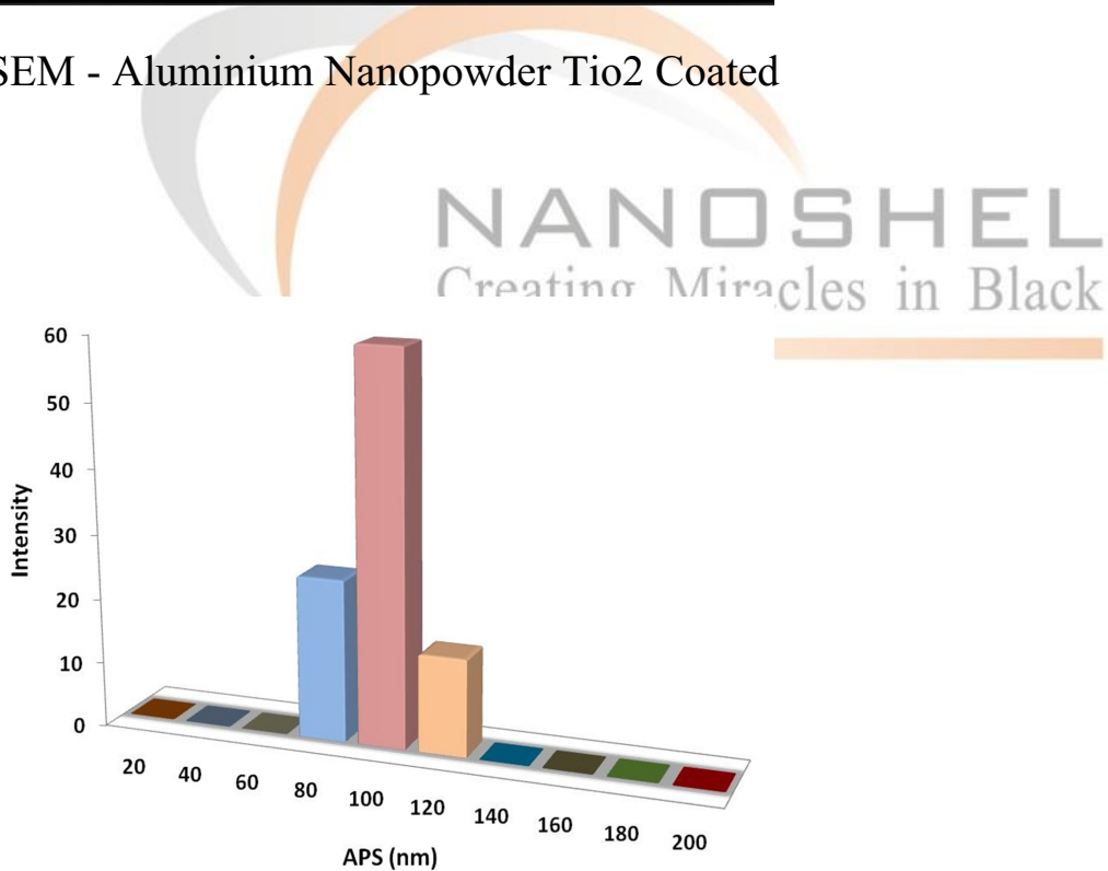
Particles Size Analysis - Al Nanopowder TiO 2 Coated
