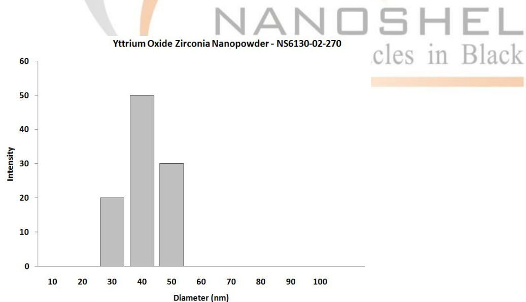
Ytria Stabilized Zirconia Nanoparticles – Size Analysis
