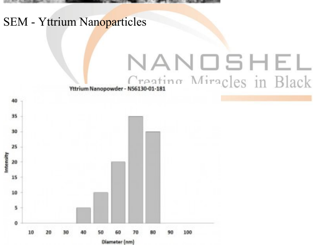
Particles Size Analysis - Y Nanopowder
