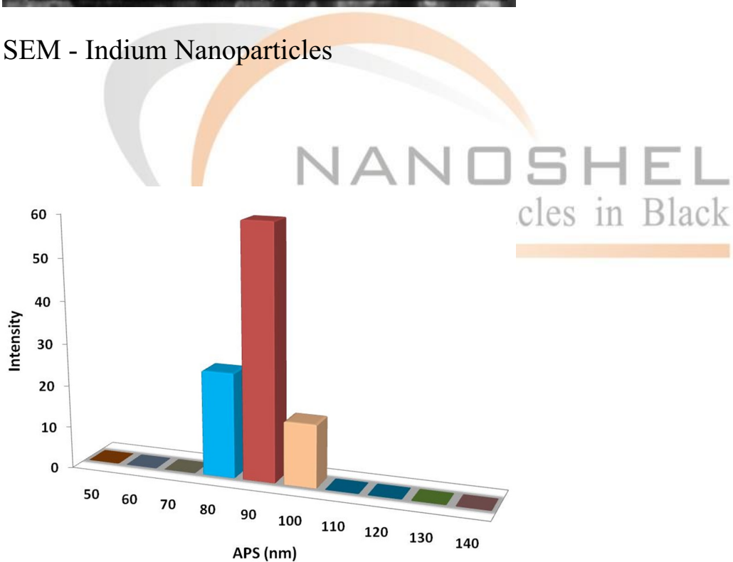
Particles Size Analysis - Indium Nanoparticles
