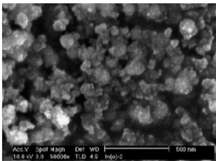
SEM - Indium Nanoparticles
