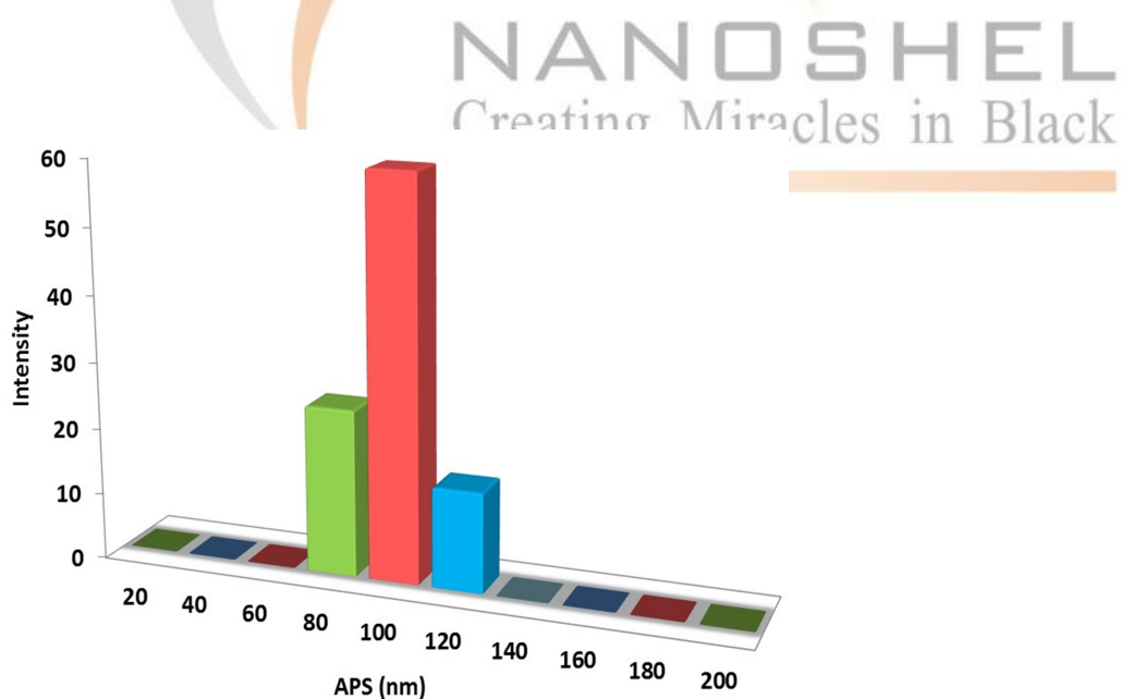
Particles Size Analysis - Lithium Nanopowder
