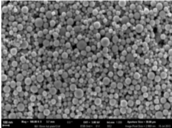
SEM - Vanadium Nanoparticles
