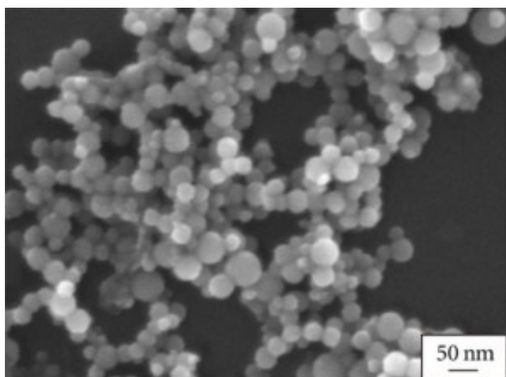
SEM - Silver Coated Aluminum Nanopowder
