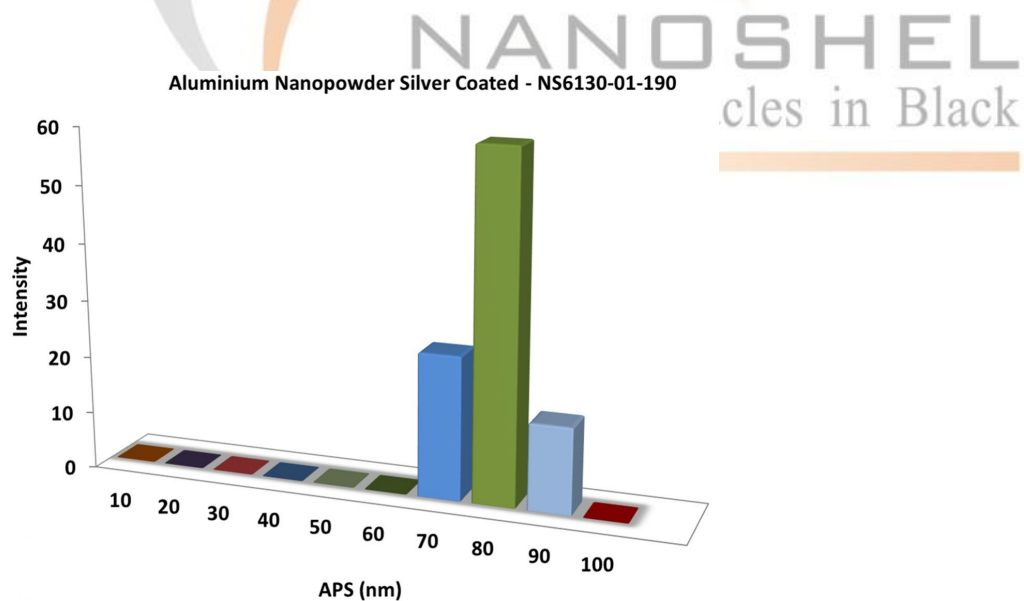
Particles Size Analysis - Al nanopowder
