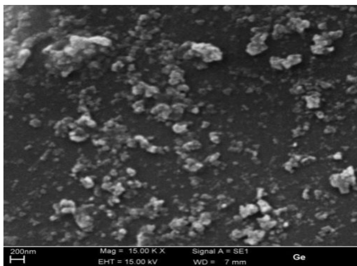
SEM - Germanium Nanopowder
