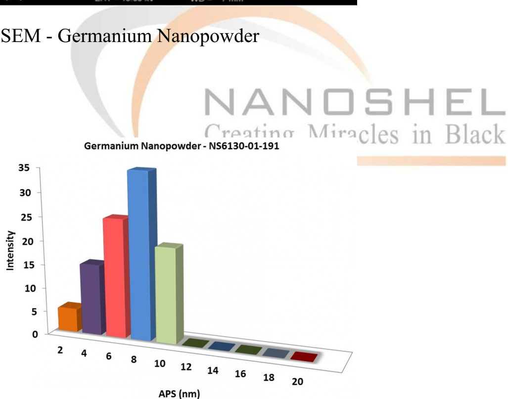
Particles Size Analysis - Ge Nanopowder
