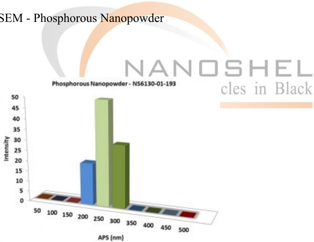
Particles Size Analysis - P Nanoparticles
