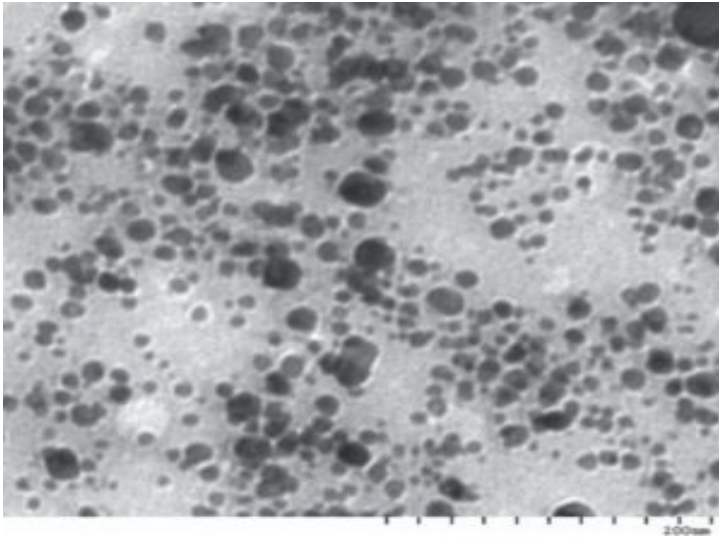
SEM - Phosphorous Nanopowder
