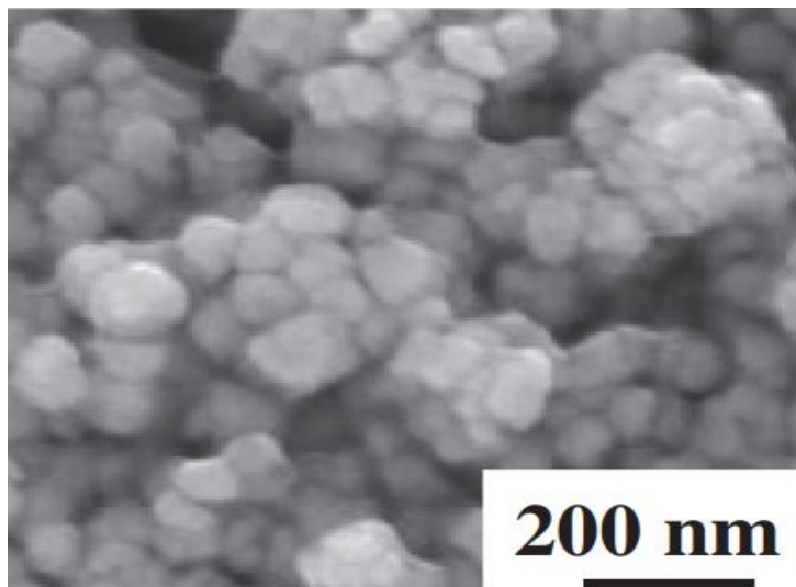
SEM – NiC Nanoparticles
