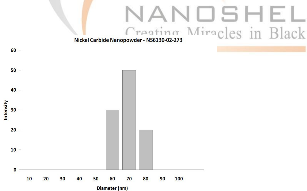
Nickel Carbide Nanoparticles – Size Analysis
