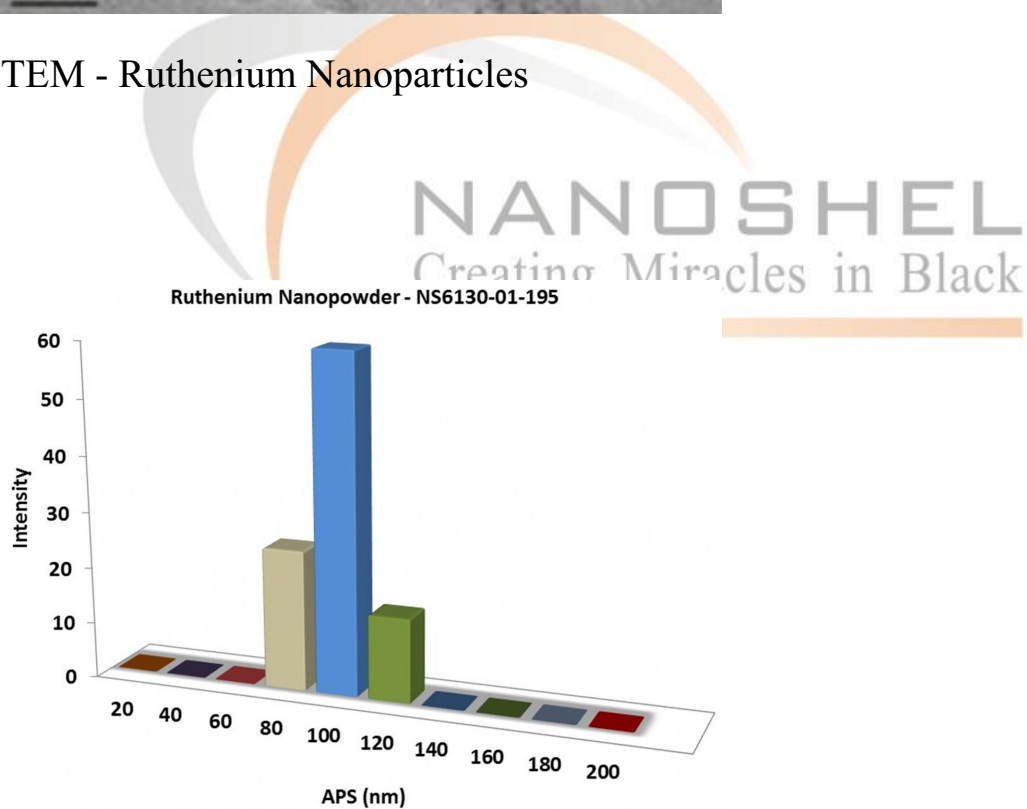
Particles Size Analysis - Ru Nanopowder
