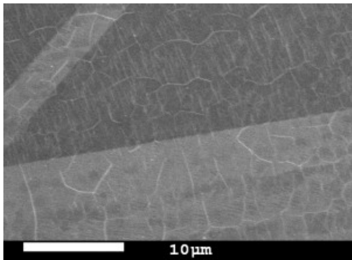
SEM-Monolayer Graphene Film
