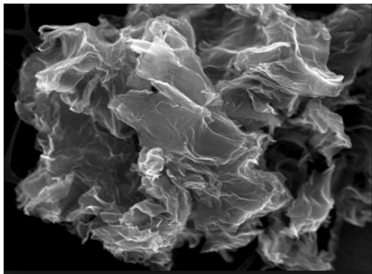
SEM-Graphite Oxide Powder
