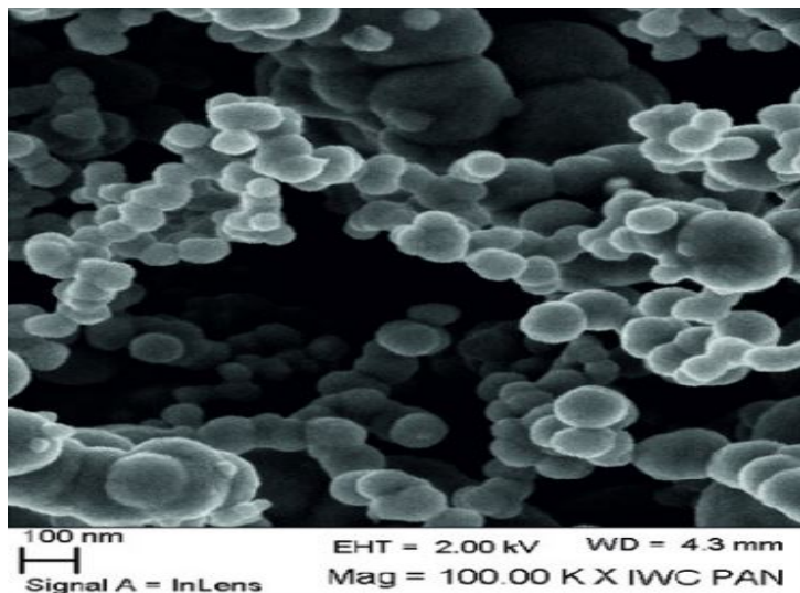
SEM - SiC Nanoparticles
