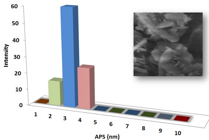
Particles Size Analysis - ZnO
