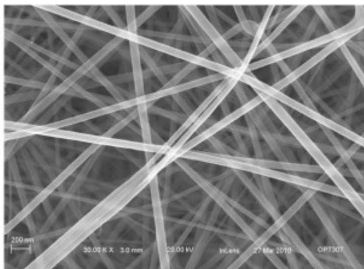
SEM - Silicon Nanowire on Silicon Wafer Substrate
