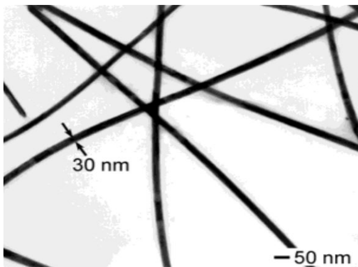
TEM - Silver Nanowire Polymer
