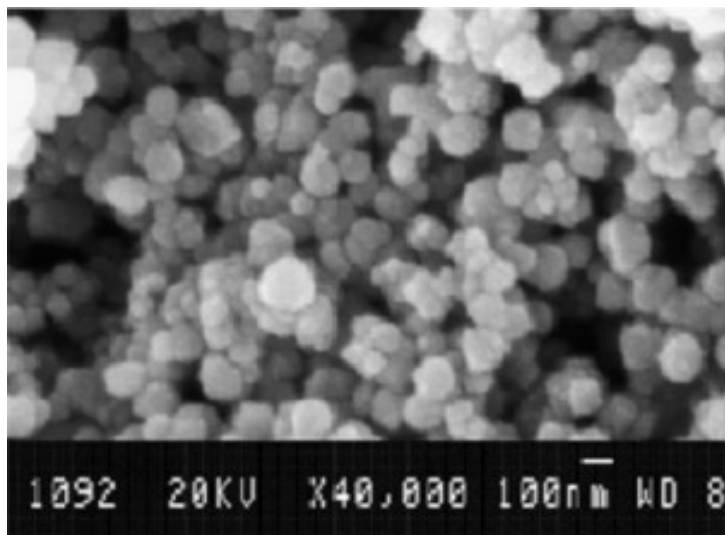
SEM - CeO 2 Nanoparticle Dispersion
