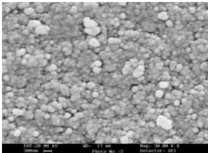
SEM - ZnO Nanoparticle
