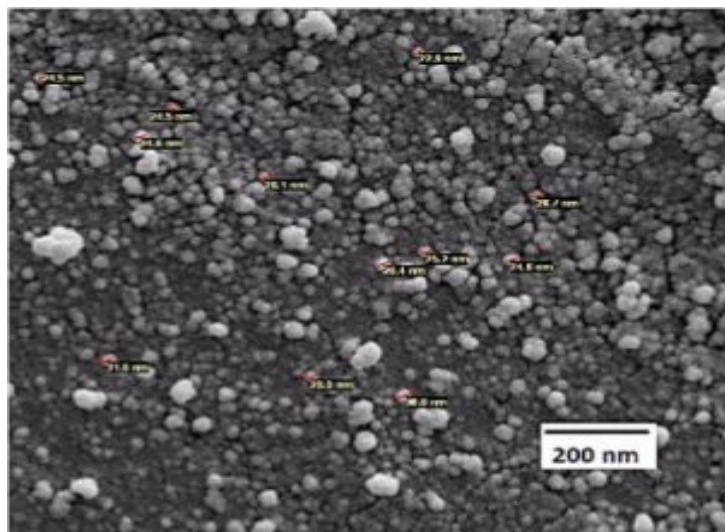
SEM - Fe 2 O 3 Nanoparticles
