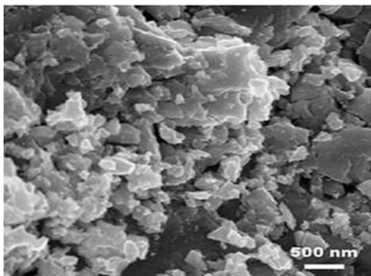
SEM – NbN Nanoparticles
