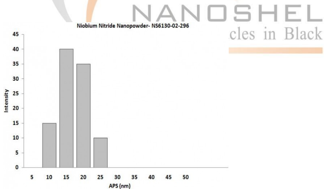
Niobium Nitride Nanopowder – Size Analysis
