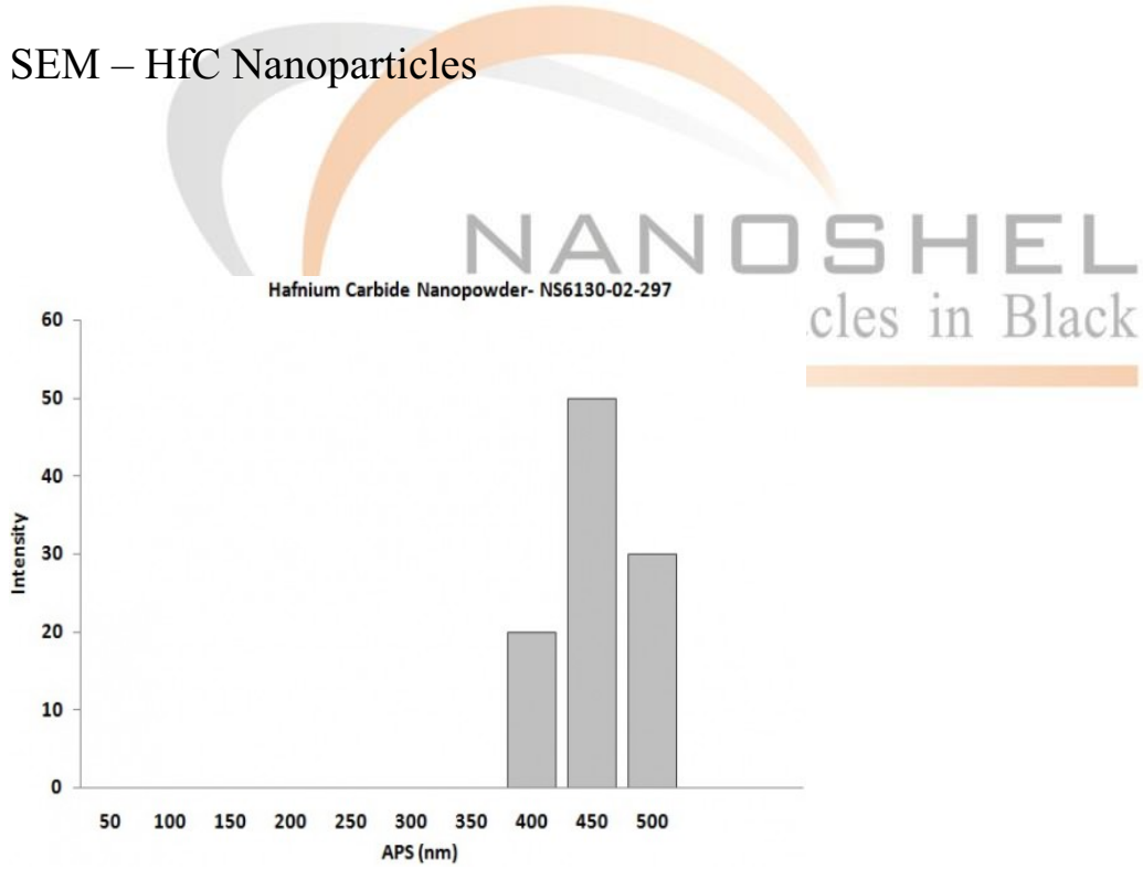
Hafnium Carbide Nanopowder – Size Analysis
