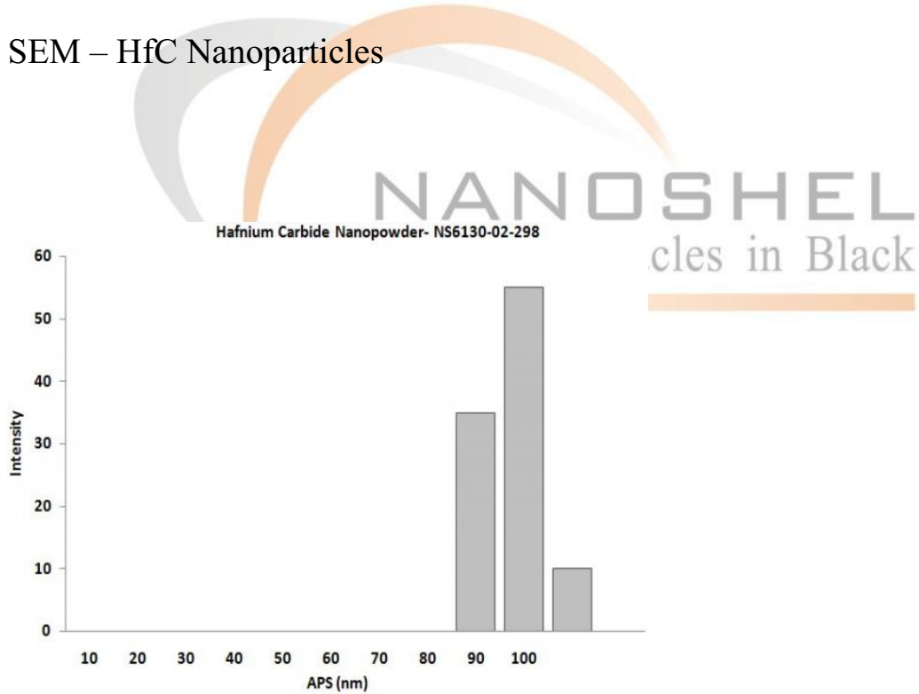
Size Analysis of Hafnium Carbide Nanoparticles
