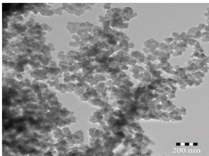
TEM - Boron Nitride Nanoparticles
