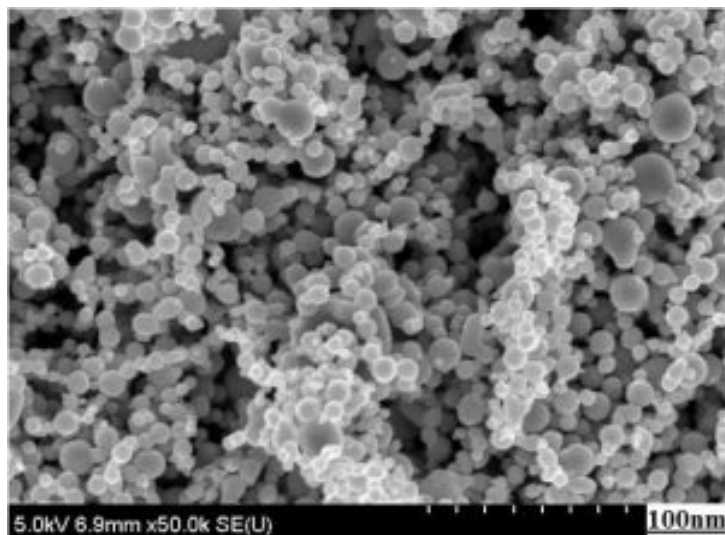
SEM - Nickel II Oxide Dispersion
