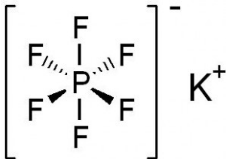
Potassium-Hexafluorophosphate-Structure-300x212
