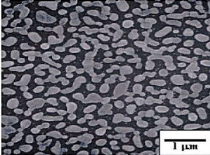
SEM-Titanium Silicide Powder
