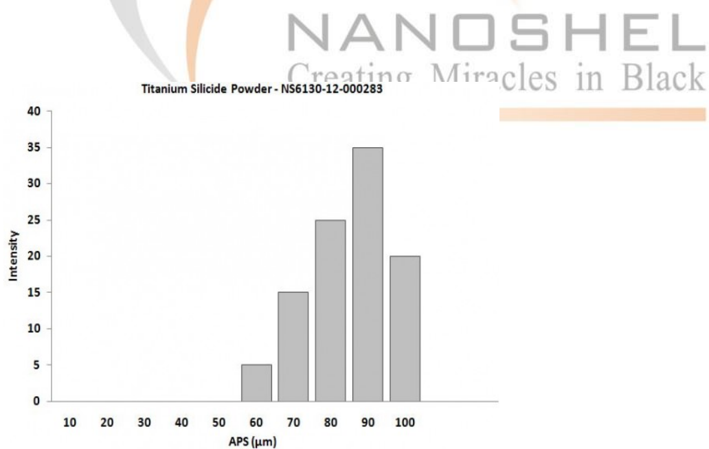
Particles Size of Analysis-Titanium Silicide Powder
