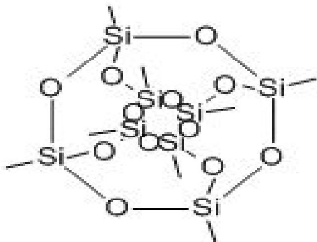
Octamethyl POSS
