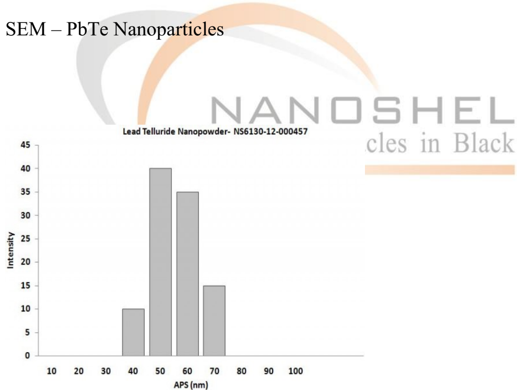
PbTe Nanoparticles – Size Analysis
