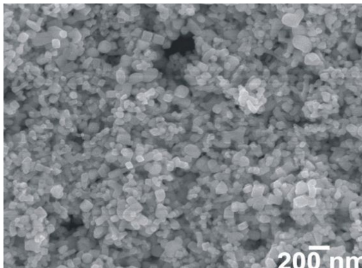
SEM - PbTe Nanoparticles
