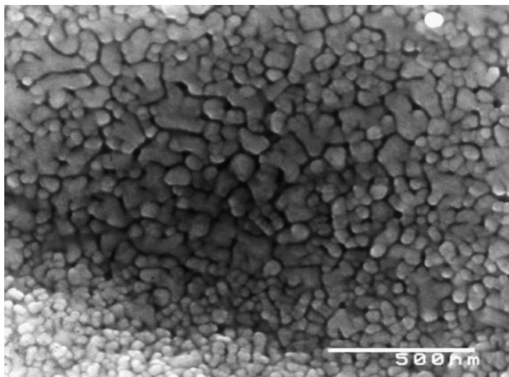
SEM - LaCoO 3 Nanoparticles
