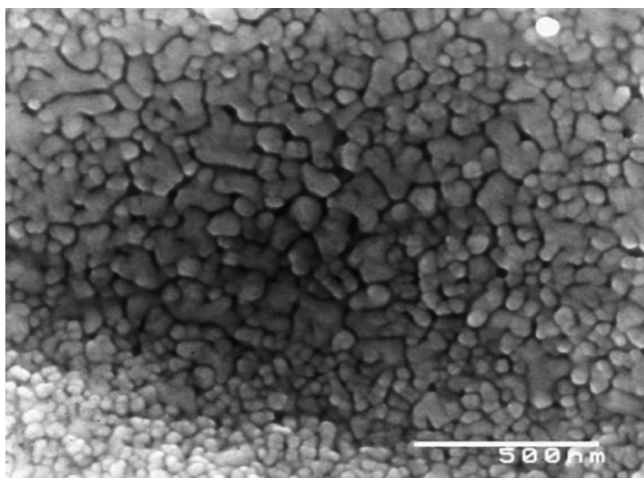
SEM – Lanthanum Cobaltite Nanoparticles
