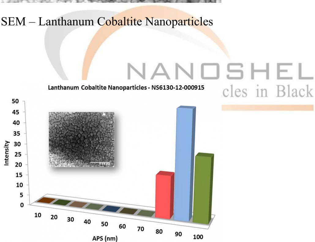
Particles Size Analysis – LaCoO 3 Nanopowder
