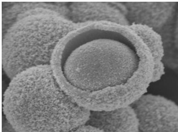
SEM - Ag SiO 2 Core Shell Nanoparticles
