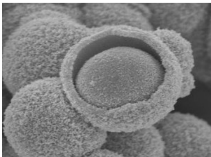
SEM - Aluminium Silicon Oxide Core Shell
