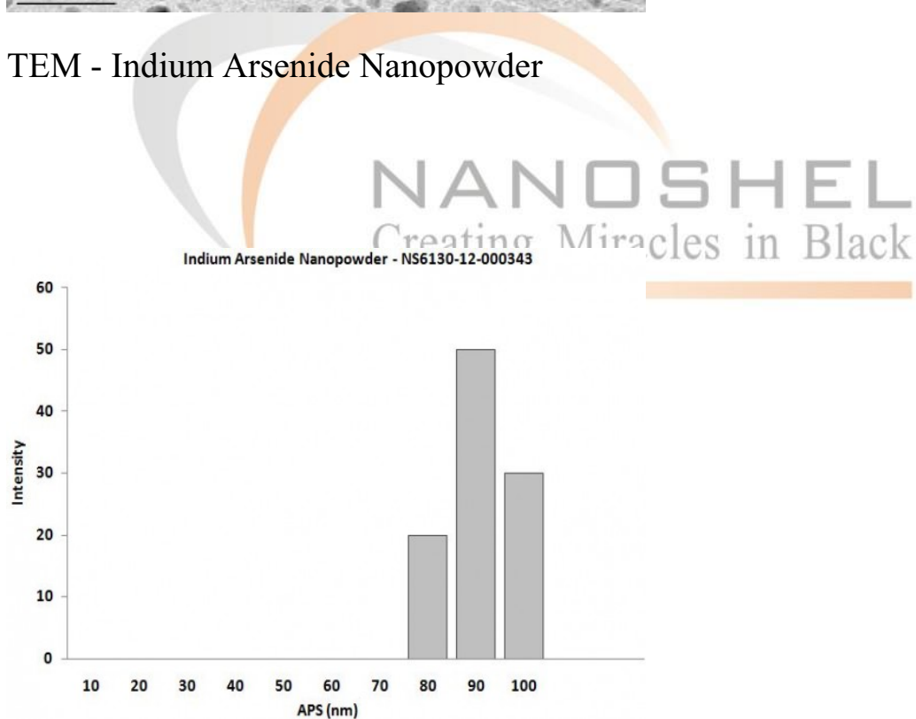
Particles Size Analysis - Indium Arsenide Nanopowder
