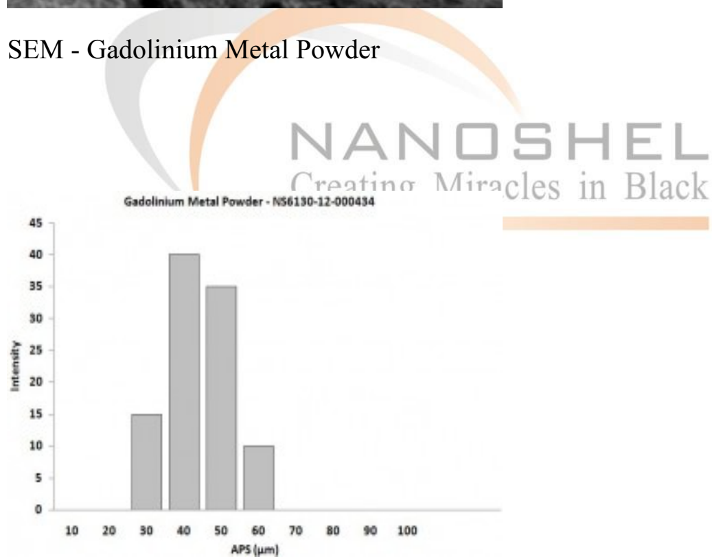
Particles Size Analysis - Gadolinium Metal Powder
